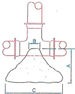
TEES AND TAPPING SLEEVE
