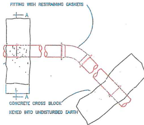
VERTICAL DOWN BEND NOT TO SCALE
