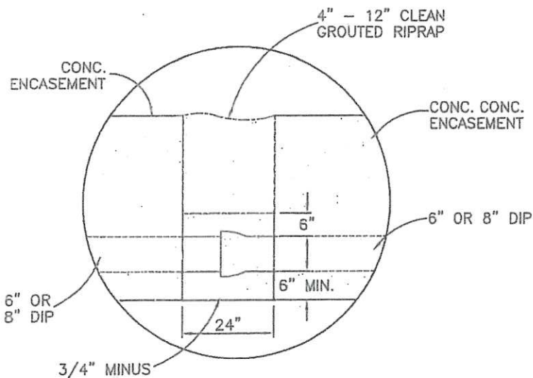
DETAIL "A" TYPICAL JOINT IN PIPE OR FITTING
