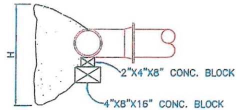
TYPICAL SECTION
